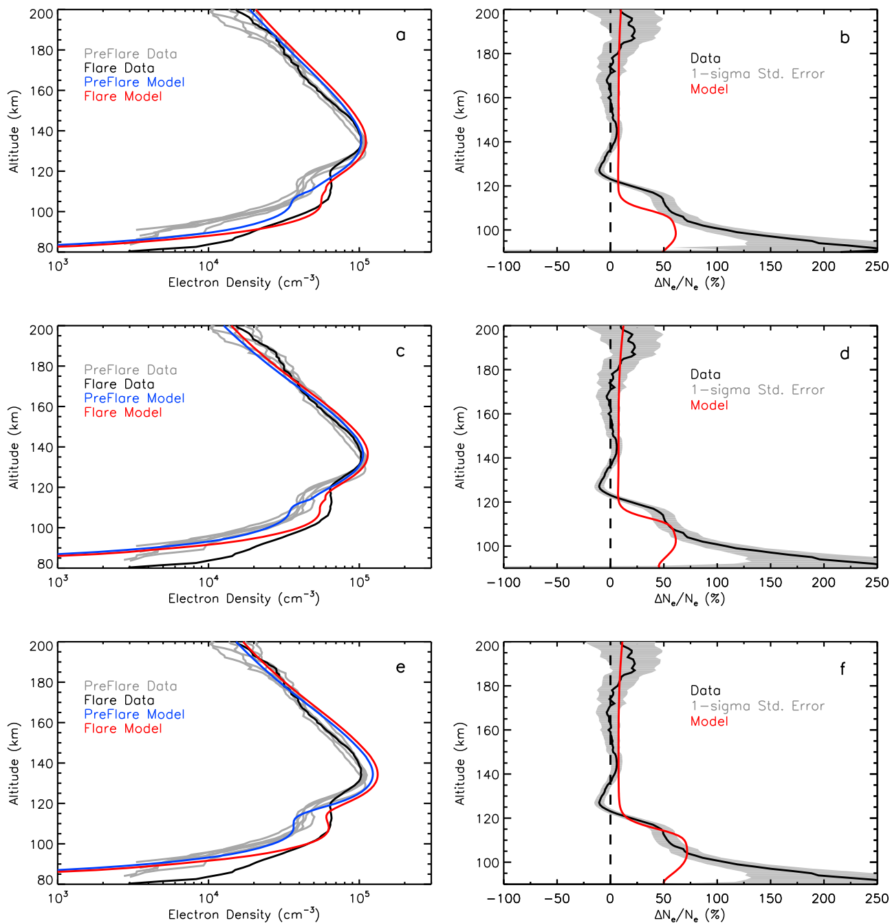
Figure 6. April 15 profiles of (left) simulated and observed electron density and (right) percentage difference between flare-affected and average background profiles, as in Figure 3. Figures 6a and 6b show results using the same model parameters as Mendillo et al. [2011]. Figures 6c and 6d show results with an alternate neutral temperature profile (section 3.1). Note the change in altitude of the modeled electron density peaks in between Figures 6a and 6c. Figures 6e and 6f show the best and final results, which use both the alternate temperature profile and an alternate parameterization for the secondary ionization ratio with W = 28 eV (section 3.2). Note the change in altitude of the sudden increase in the percentage difference profile between Figures 6d and 6f.
