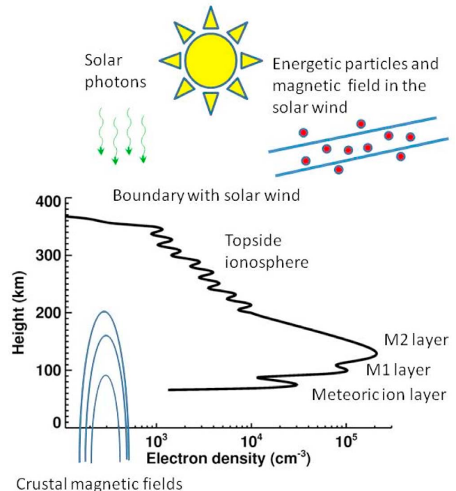
Figure 2. Schematic illustration of the main features and forcings associated with the ionosphere of Mars. Reproduced from Withers [2011]. Reprinted with permission.
