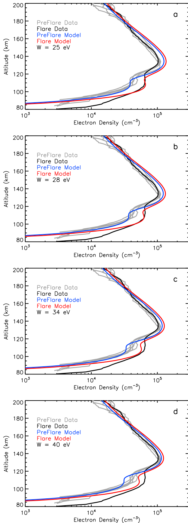
Figure 7. Simulated and observed electron density profiles for the 15 April flare. Each plot shows results for a different value of W used in the secondary ionization parameterization: (a) 25 eV, (b) 28 eV, (c) 34 eV, and (d) 40 eV. Note that as W is increased, the modeled electron density at the peaks decreases.
